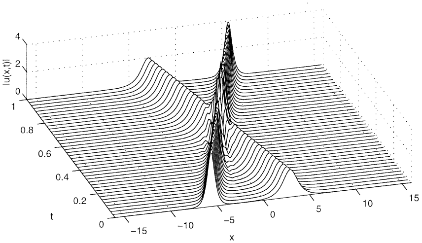
FIG. 6. Two-soliton solution for NLS, in magnitude.
