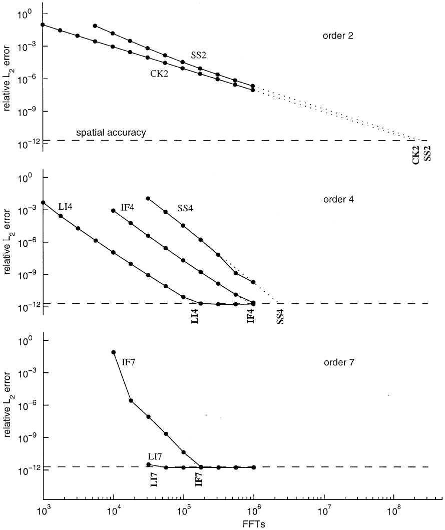
FIG. 8. Performance for KdV. For clarity, methods are grouped by order. Actual data are shown as filled circles; linear extrapolations are shown as dotted lines. The goal is to match spatial resolution (dashed lines) with as little cost (measured by counting FFTs) as possible. The point at which a method is estimated to achieve this matching is indicated by a boldface vertical label.
