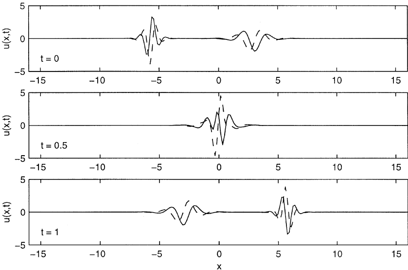
FIG. 7. Snapshots of real (solid) and imaginary (dashed) parts of the NLS solution of Fig. 6.
