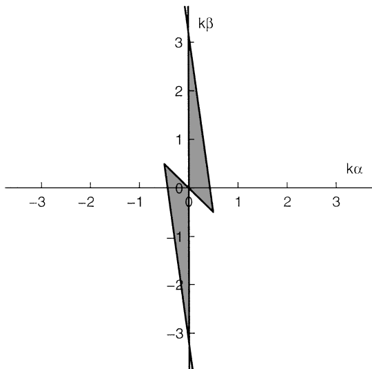
FIG. 3. Stability region for the linearly implicit AB4/AM2 method. The shaded portion indicates time stability of the method for choices of time step k and parameters \alpha and \beta in (5).
